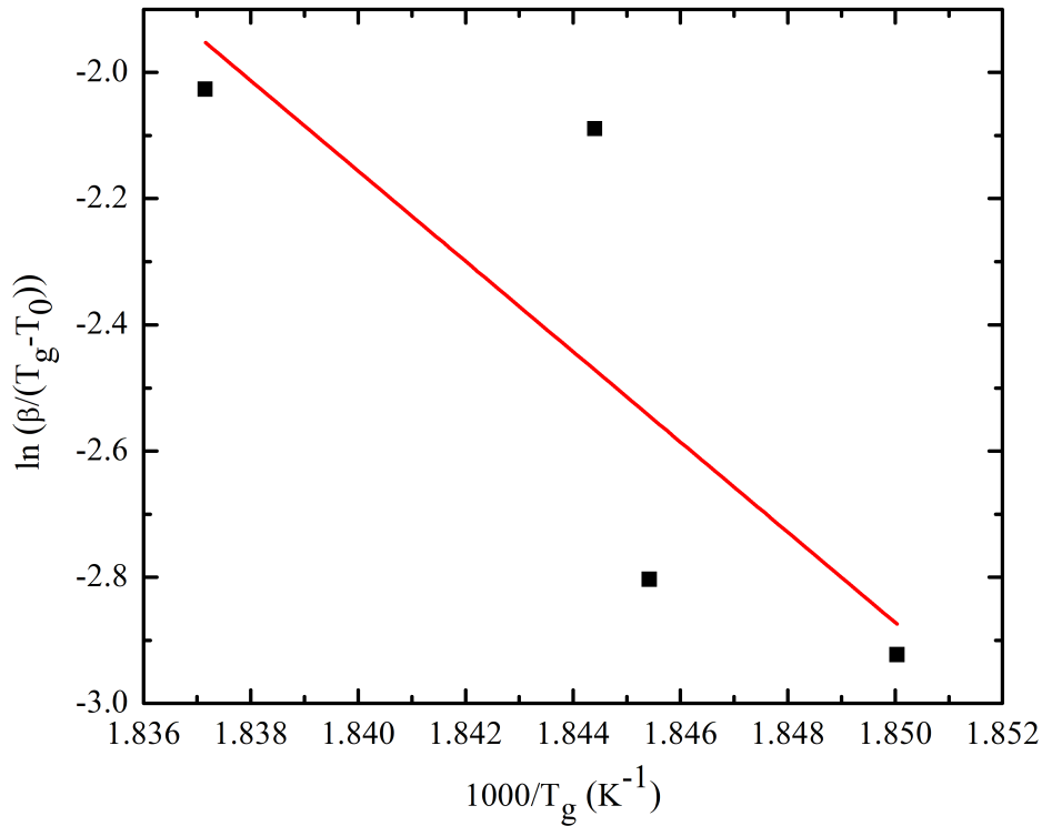
Figure 5.3: Augis-Bennett plot for ZBLAN glass
