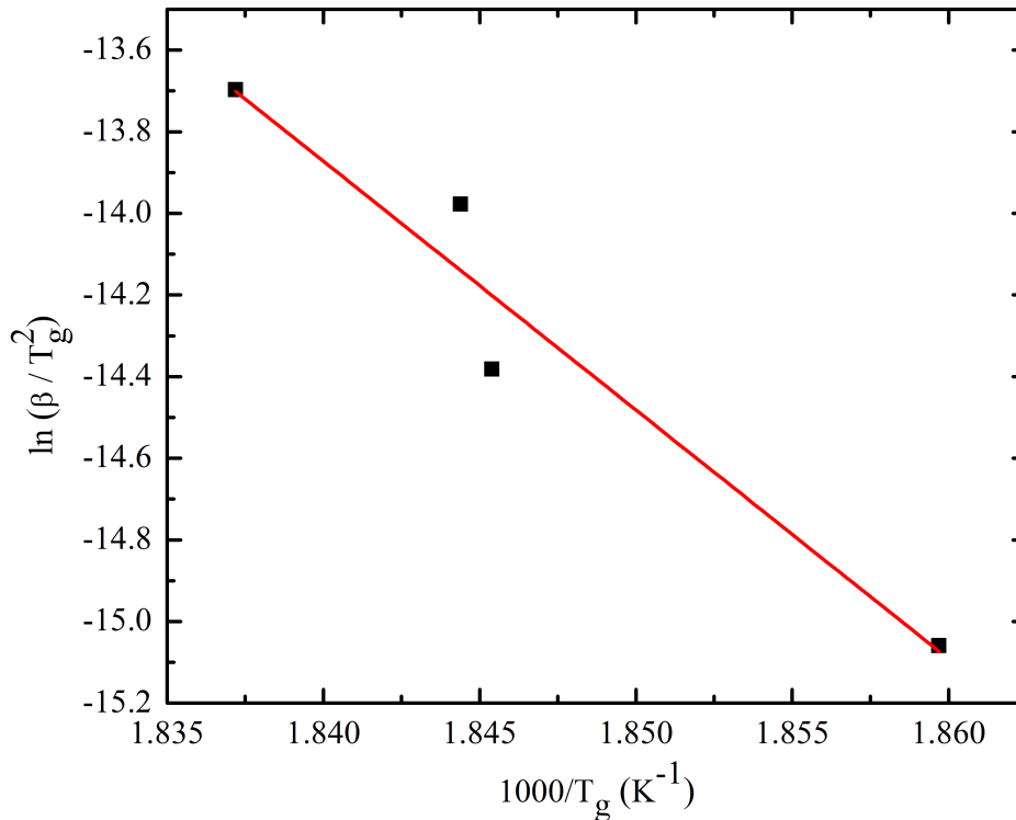
Figure 5.2: Kissinger plot for ZBLAN glass
